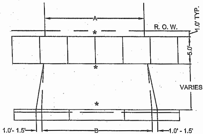
DRIVE APPROACH WITH SIDEWALK
