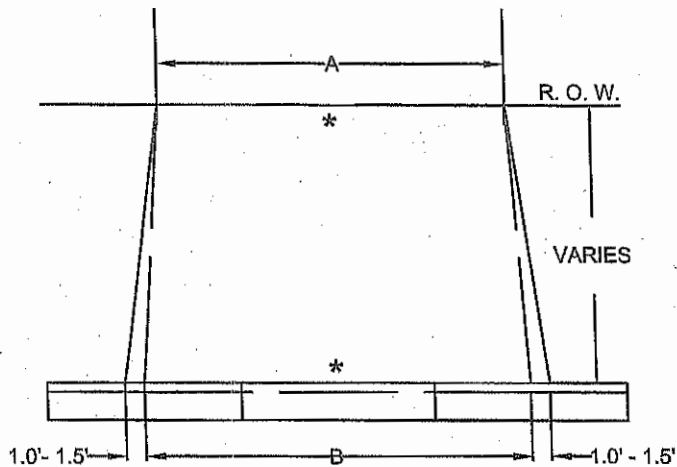
DRIVE APPROACH WITHOUT SIDEWALK
